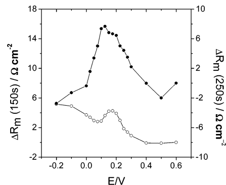
Figure 2. Evolution of the motional resistance calculated at steady-state conditions. Data of K_4Fe_4[Fe(CN)_6]_x \cdot mH_2O material deposited applying a controlled cathodic current of 40 \mu A \cdot cm^{-2} (○) during 150 s and (●) during 250 s.
