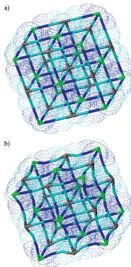
Figure 4. (a) Structure of Prussian Blue hexacyanoferrate. (b) ES crystalline structure proposed theoretically. It is believed that the vacancies in the Fe'(CN) 6 site are surrounded by water molecules (Fe'(CN) 6-m m(H 2 O) sites), whose stoichiometry is very difficult to be determined. Interstitial alkali metals were omitted for clarity. Green sticks correspond to Fe(III) atoms, black sticks correspond to Fe(II) atoms, blue sticks correspond to nitrogen atoms, and cyan sticks correspond to carbon atoms.
